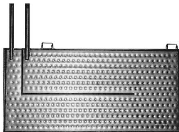
Mueller Temp-Plate serpentine pattern.
