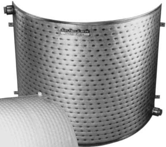
Shell Clamp-Ons
