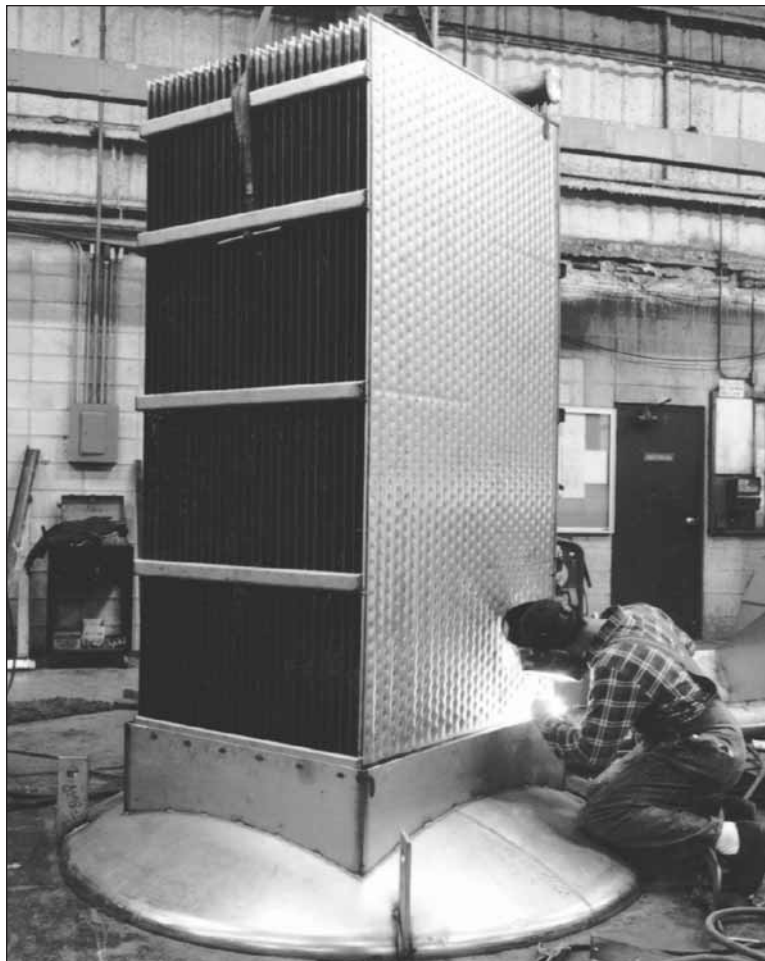
Inflated Temp-Plate bank assembly for heat recovery from hot gas.
