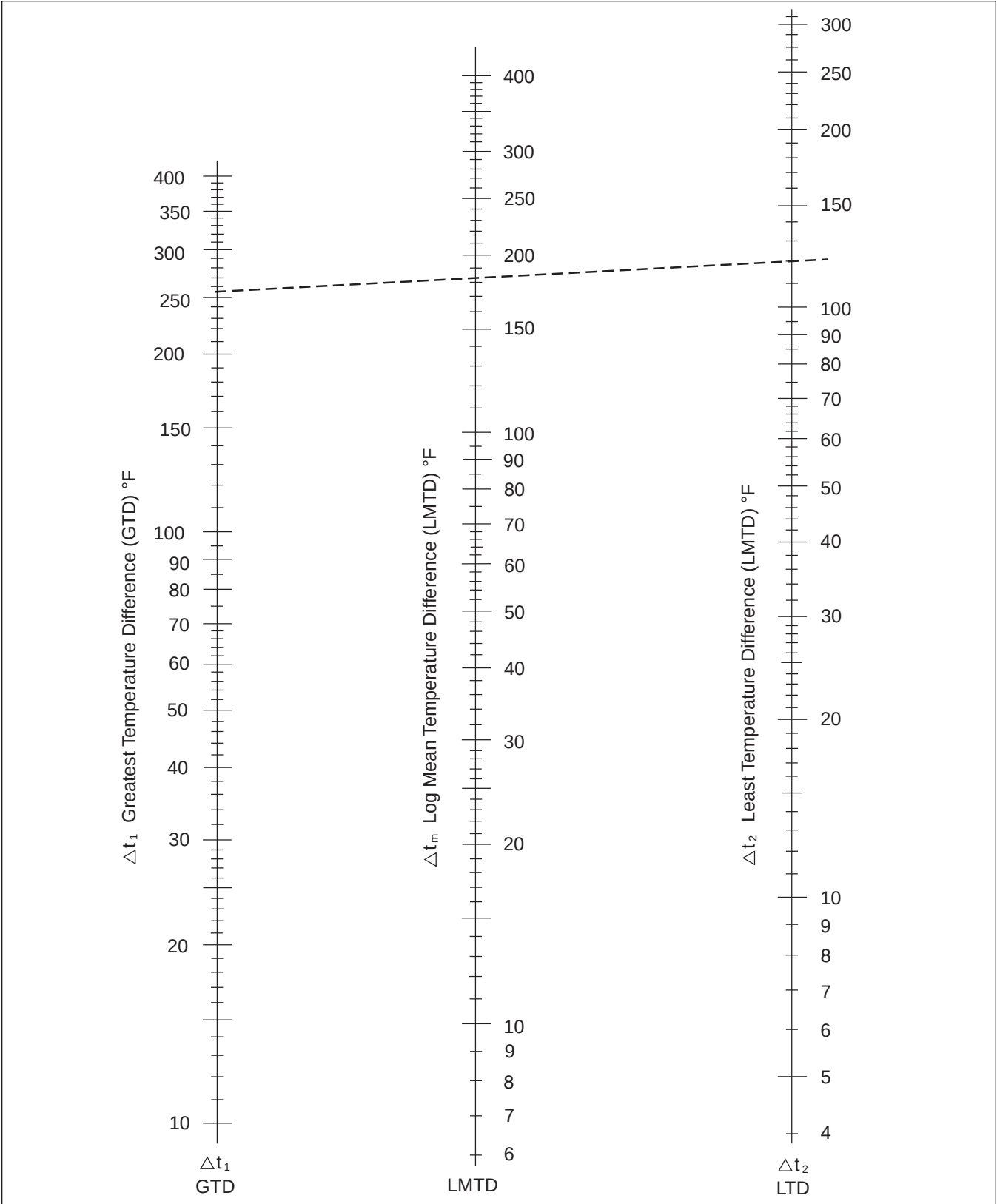
LOGARITHMIC MEAN TEMPERATURE DIFFERENCE NOMOGRAPH
